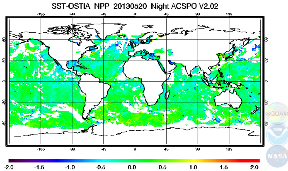
Figure 3-5 – Nighttime global composite map of ACSPO VIIRS SST – OSTIA for 20 May 2013
