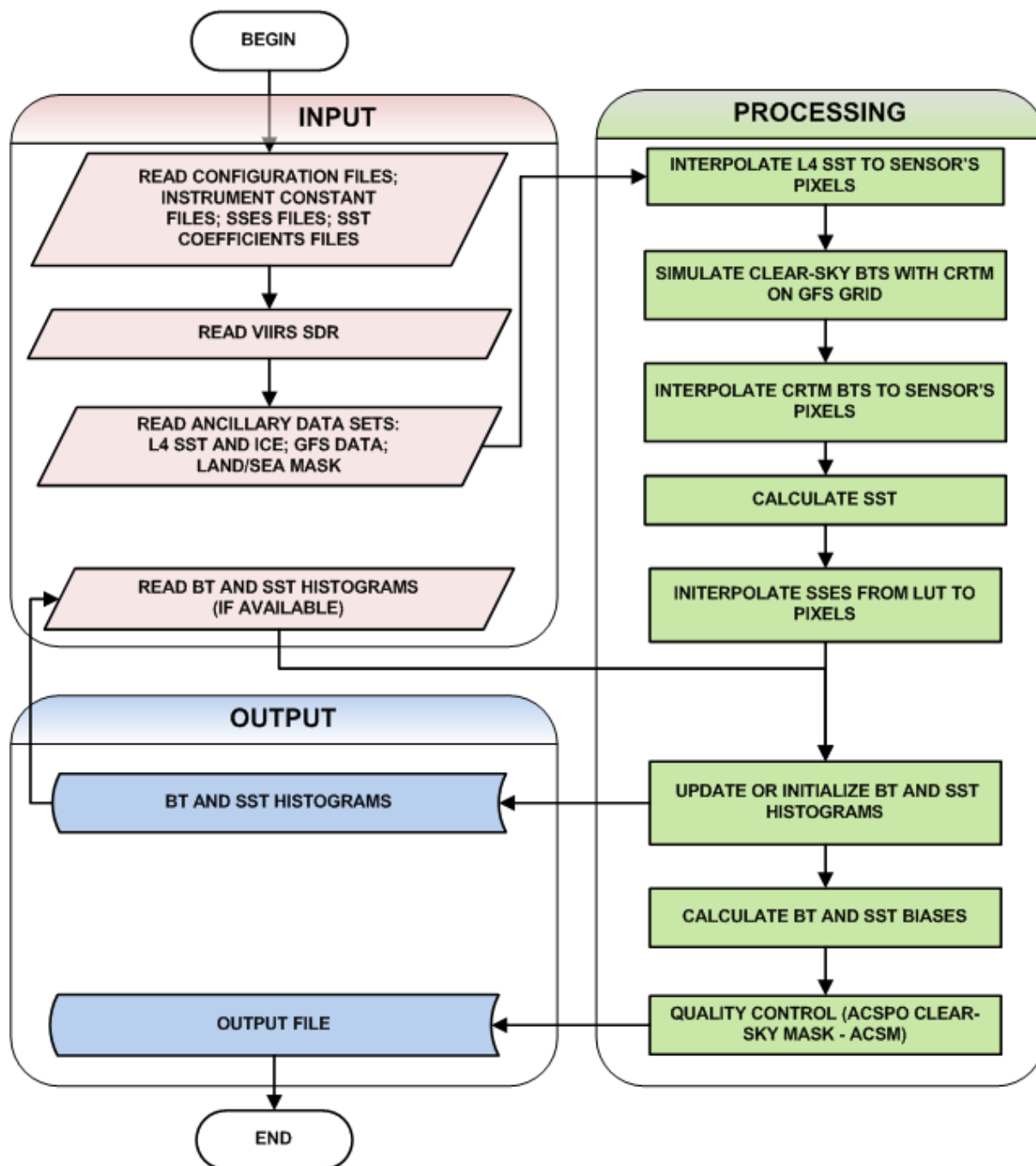
Figure 2-1 – Flow Chart of ACSPO Data Processing
