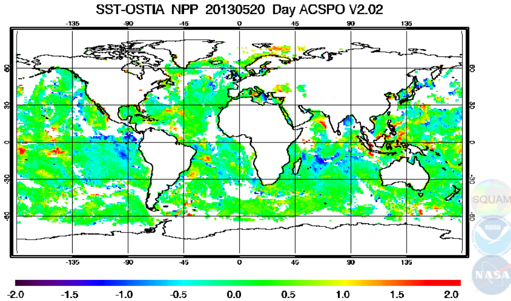
Figure 3-4 – Daytime global composite map of ACSPO VIIRS SST – OSTIA for 20 May 2013
