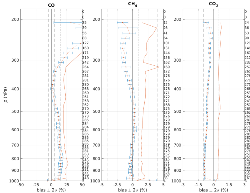
Figure 1. NOAA-20 NUCAPS carbon trace gas profile retrieval statistics (cf. Nalli et al. 2020). Shown are bias (dotted red line) and precision (1 \sigma variability; solid red line) versus ATom-4 in situ aircraft data (NOAA/GML measurements): (left) carbon monoxide, (center) methane, and (right) carbon dioxide. Layer sample sizes are indicated on the right margins. More details can be found in the NUCAPS validated maturity review from the STAR JPSS - Algorithm Maturity Matrix .
