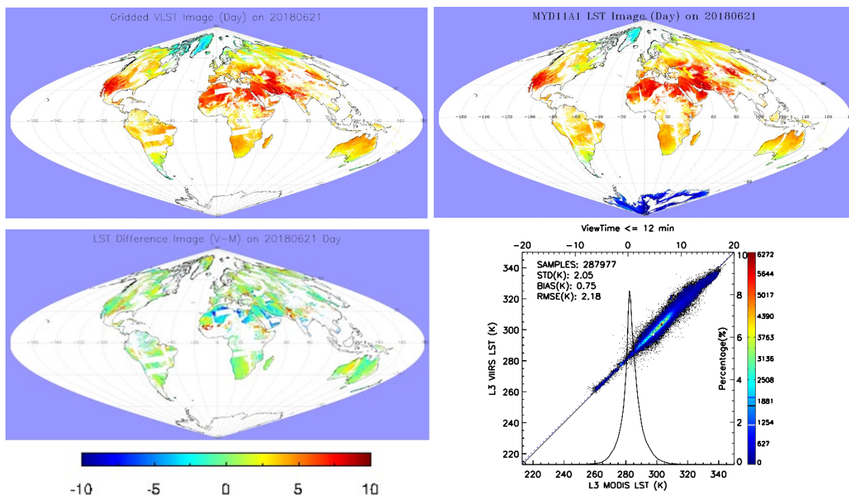
Figure 4-1 Cross comparison: daytime case on June 21, 2018
