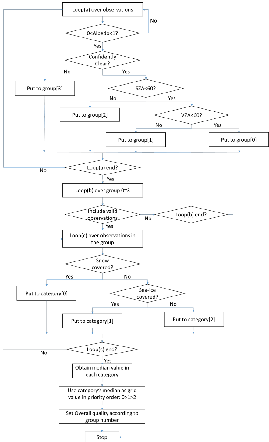
Figure 2-6 Pixel-level processing flowchart in the composition algorithm.
