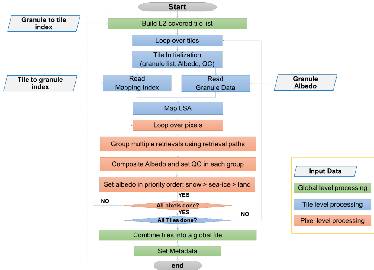
Figure 2-5 High Level Flowchart of the LSA production for illustrating the main processing steps. Note that the detailed content of pixel-level processing is illustrated in Figure 2-6.
