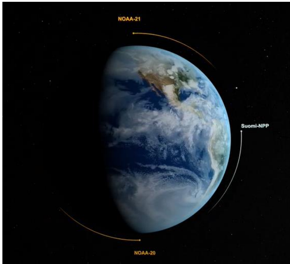
Figure 2-16. NOAA-21, SNPP, and NOAA-20 follow the same orbit with NOAA-21 leading S-NPP and NOAA-20 by about 25 and 50 minutes, respectively (from https://www.nesdis.noaa.gov/our-satellites/currently-flying/joint-polar-satellite-system ).
