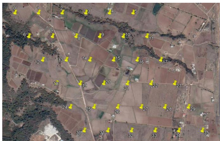
(b) Cropland (North America)
