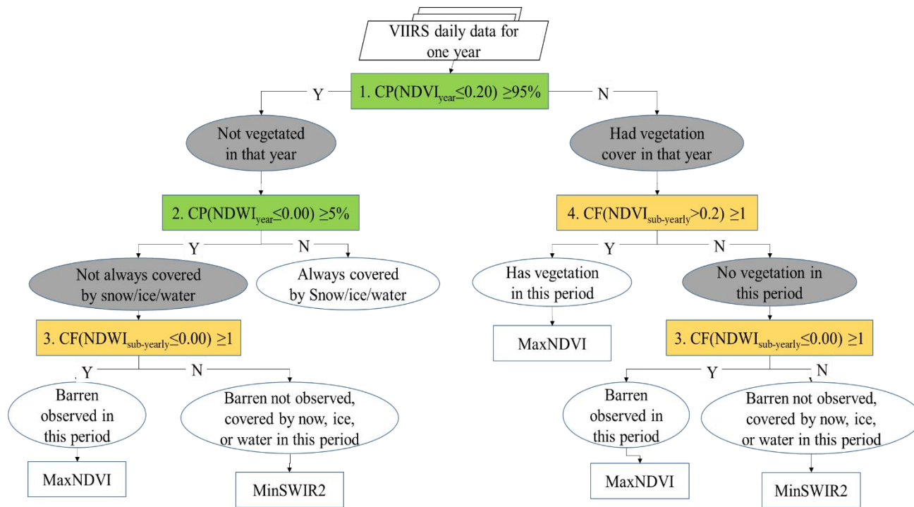
Figure 2-7. A flowchart of the decision rules and compositing criteria used in the SA-Comp method. CP is the cumulative percentage of observations in a year that meet the conditional statement in the parentheses, whereas CF is the cumulative frequency within a specific compositing period.
