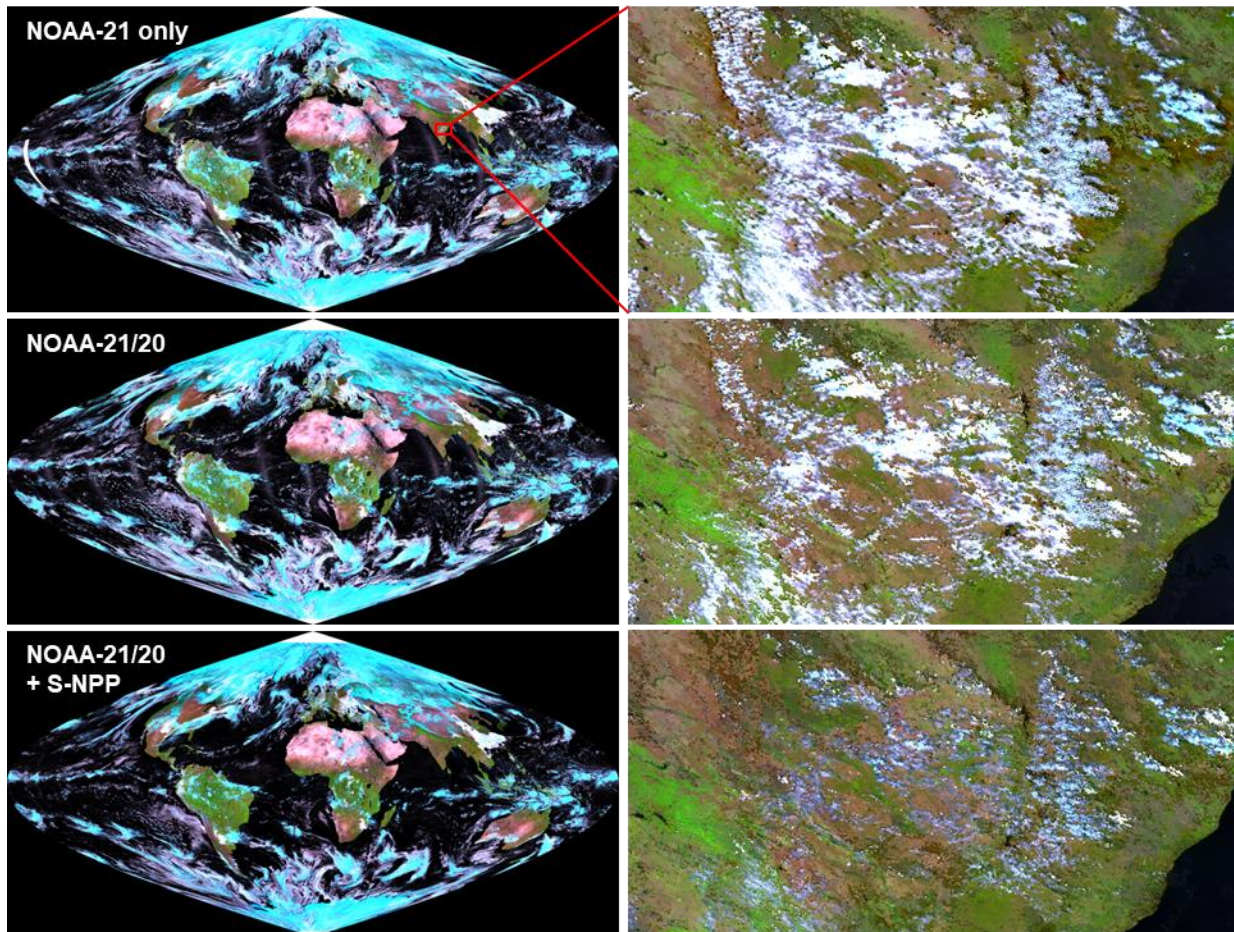
Figure 2-6. Example global daily mosaics created using all surface reflectance data acquired by one or more VIIRS-carrying satellites on March 15, 2024 (left). The zoom-in views over eastern India (right) show that use of more than one satellites may reduce cloud cover under certain circumstances.
