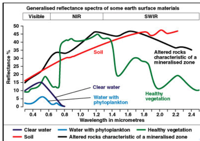
Figure 2-5. Laboratory measured spectra of selected surface types (Based on spectral data from https://speclab.cr.usgs.gov/spectral.lib06/ds231/index.html ).
