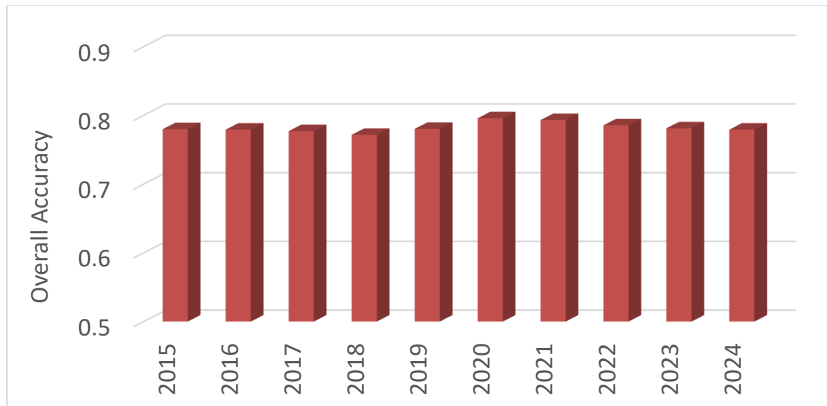
Figure 2-15. Overall accuracies of VIIRS AST products derived since 2015.
