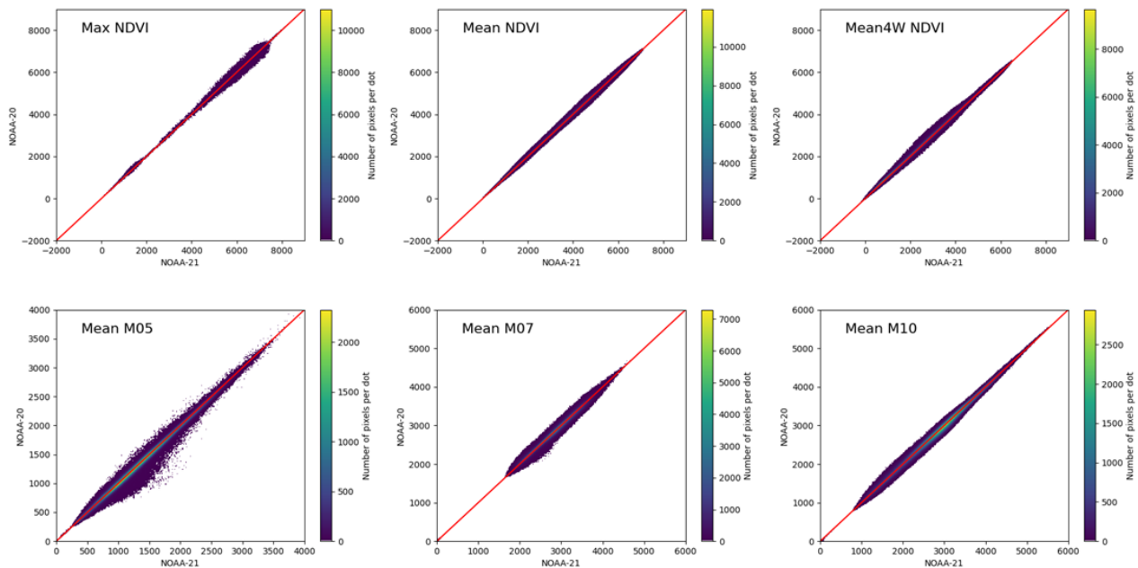
Figure 2-19. Comparison of selected annual metrics generated using NOAA-20 and “NOAA-21” data for a 12-month period (May 2023-April 2024) over southwest US (MODIS tile h09v05). The inputs for generating the “NOAA-21” annual metrics including NOAA-20 monthly composites for May 2023-October 2023, because not enough NOAA-21 surface reflectance data were available to produce monthly composites before November 2023.
