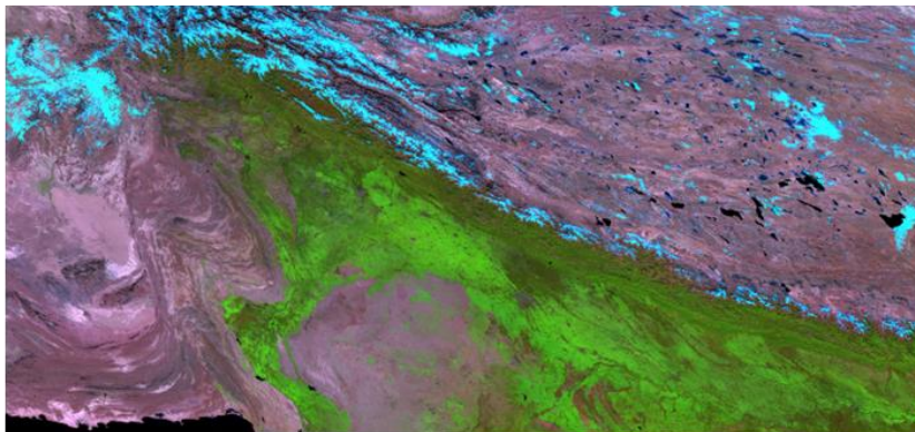
(B) Comparison of Composited SR Between NOAA-21 and NOAA-20
