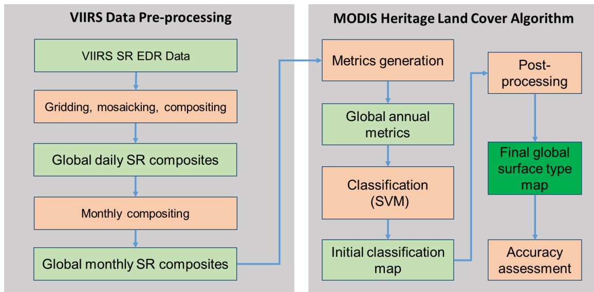
Figure 2-1. A flowchart of the processing flow of the VIIRS AST algorithm.
