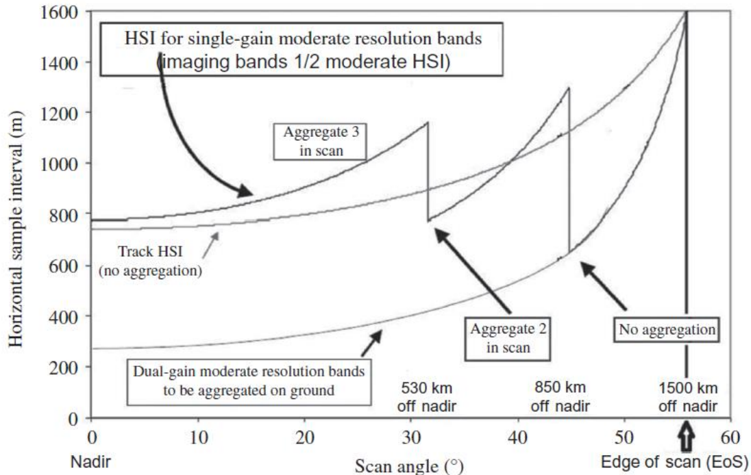
Figure 1-2. VIIRS uses a 2-stage aggregation scheme to constrain the pixel size at the end of a scan line to within about 2 times the size of a nadir pixel in the along-scan direction. Without such an aggregation scheme, a MODIS pixel at the end of a scan line is about 5 times the size of a nadir pixel in the scan direction (from (Schueler et al. 2013)).
