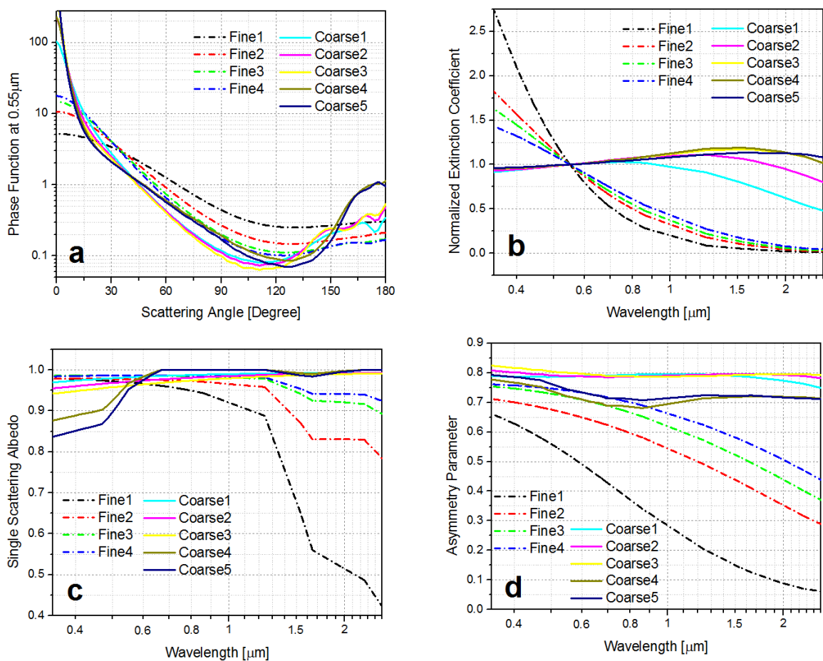
Figure 3-2. Optical properties of the candidate maritime aerosol models (four fine modes and five coarse modes): (a) phase function at 0.55μm, (b) normalized extinction coefficient (spectral extinction coefficient normalized to that at 0.55μm), (c) single scattering albedo, and (d) asymmetry parameter.
